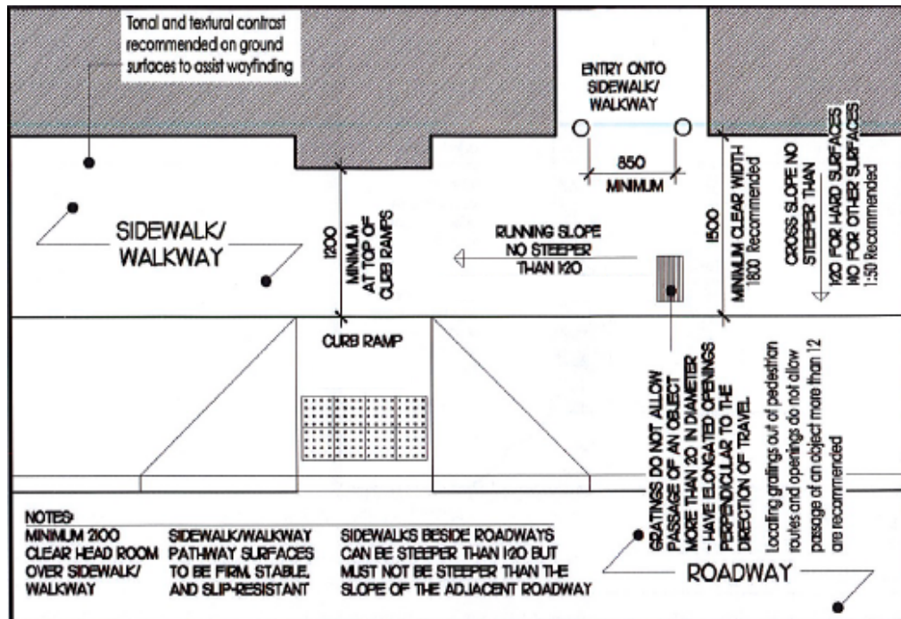
Figure 1.4 Design Requirements for Sidewalks and Walkways (Global Alliance on Accessible Technologies and Environments, 2014)
