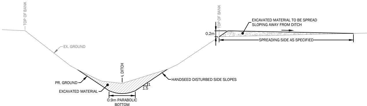
TYPICAL CLEANOUT/DITCH EXCAVATION DETAIL N.T.S.
