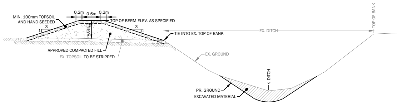
TYPICAL BERM DETAIL N.T.S.
