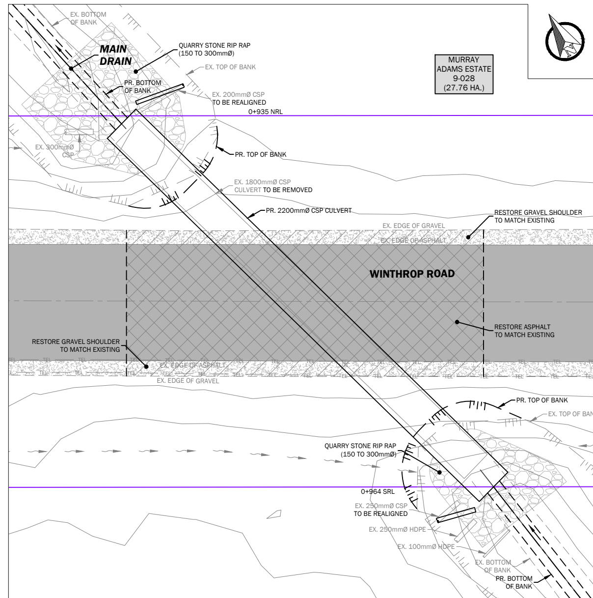
WINTHROP ROAD CROSSING DETAIL DETAIL SCALE
