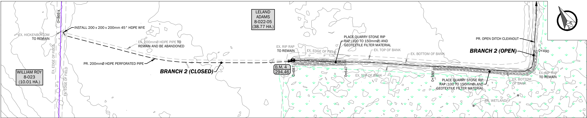
BRANCH 2 DETAIL
