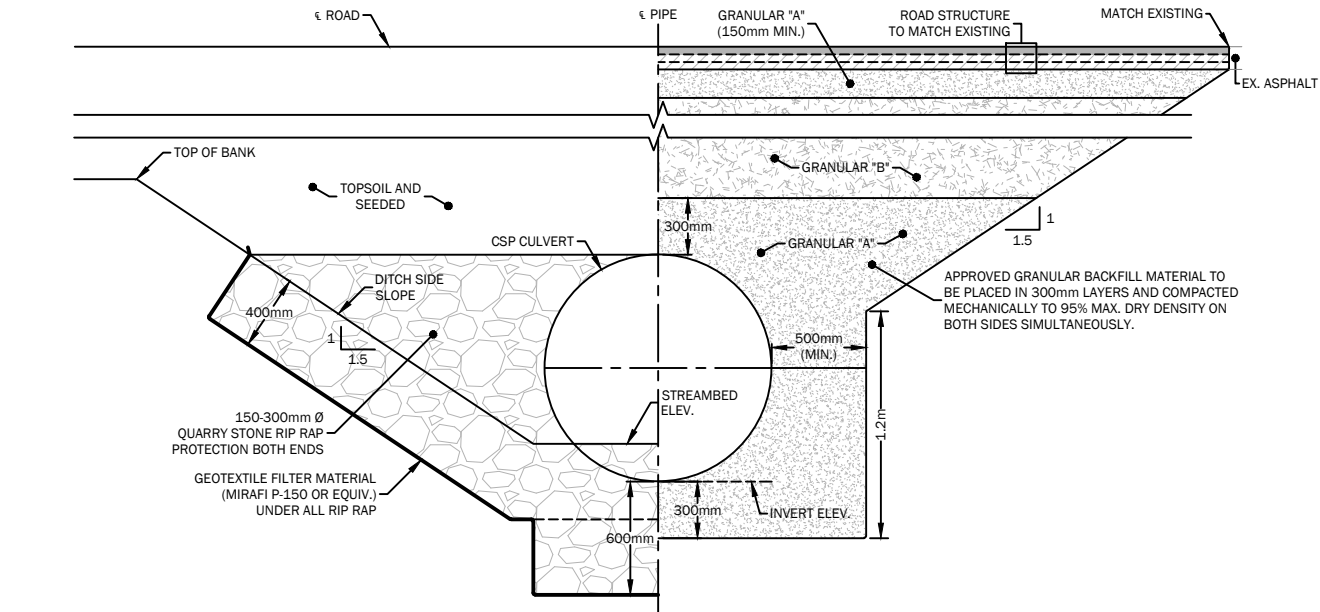
HALF ELEVATION
